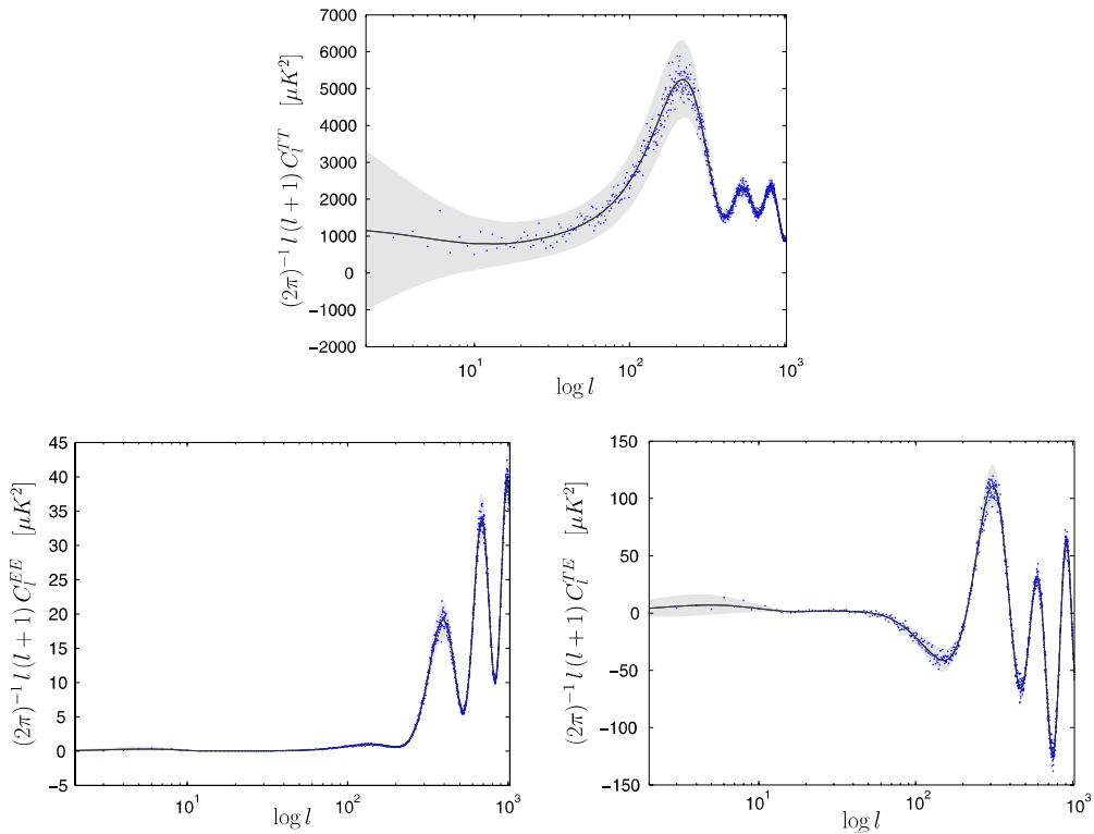
Fig. 2. CMB temperature and polarization angular power spectra C_l^{TT} (top), C_l^{EE} (bottom left), and C_l^{TE} (bottom right) of the cosmic microwave background up to a band limit L = 1024 and in \mu K^2 . Inverse and direct transforms are successively performed through the exact \mathcal{O}(L^2 \log^2 L) scalar and spin \pm 2 spherical harmonics transforms on 2L \times 2L equi-angular pixelizations on the sphere, in order to produce the estimated spectra (scattered points) from the original spectra of the concordance cosmological model (continuous lines). The original and estimated spectra coincide within the 3\sigma uncertainty defined by the cosmic variance (grey region).
