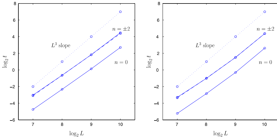
Fig. 1. Evolution of computation times t displayed as \log_2 t - \log_2 L for the direct (left) and inverse (right) spin-weighted spherical harmonics transforms of spins n = 0 (continuous line), n = +2 (continuous line), and n = -2 (dashed line). Computation times are measured in seconds on a 2.20 GHz Intel Pentium Xeon CPU with 2 Gb of RAM memory, and reported for the band limits L \in \{128, 256, 512, 1024\} . The \mathcal{O}(L^2 \log^2 L) asymptotic complexity is clearly illustrated when compared to an \mathcal{O}(L^3) slope (dotted line).
